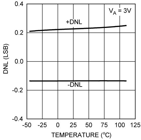
3V DNL vs. Temperature
