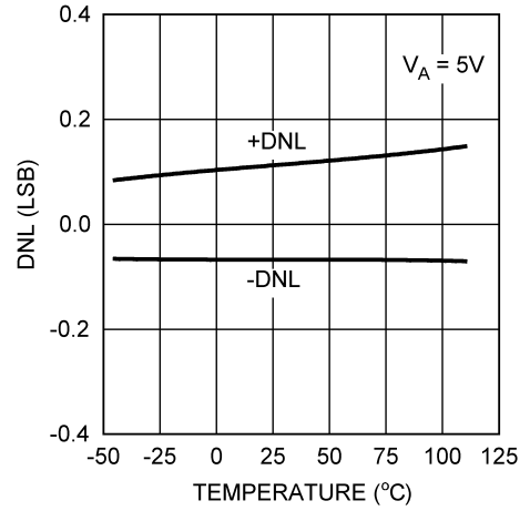
5V DNL vs. Temperature
