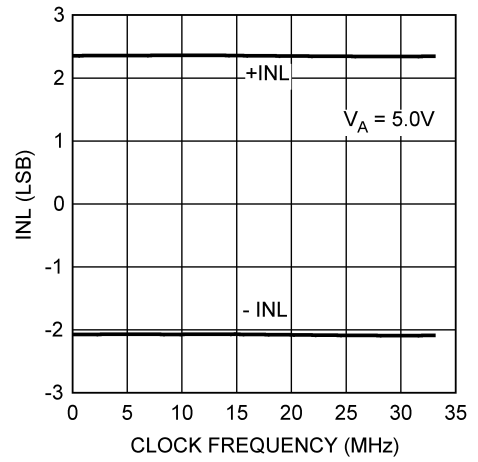
5V INL vs. f_{SCLK}
