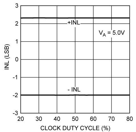
5V INL vs. Clock Duty Cycle
