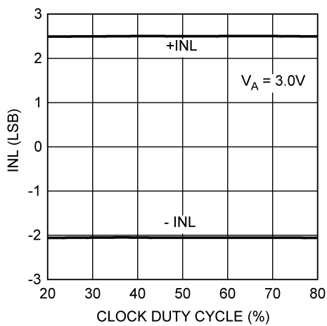
3V INL vs. Clock Duty Cycle
